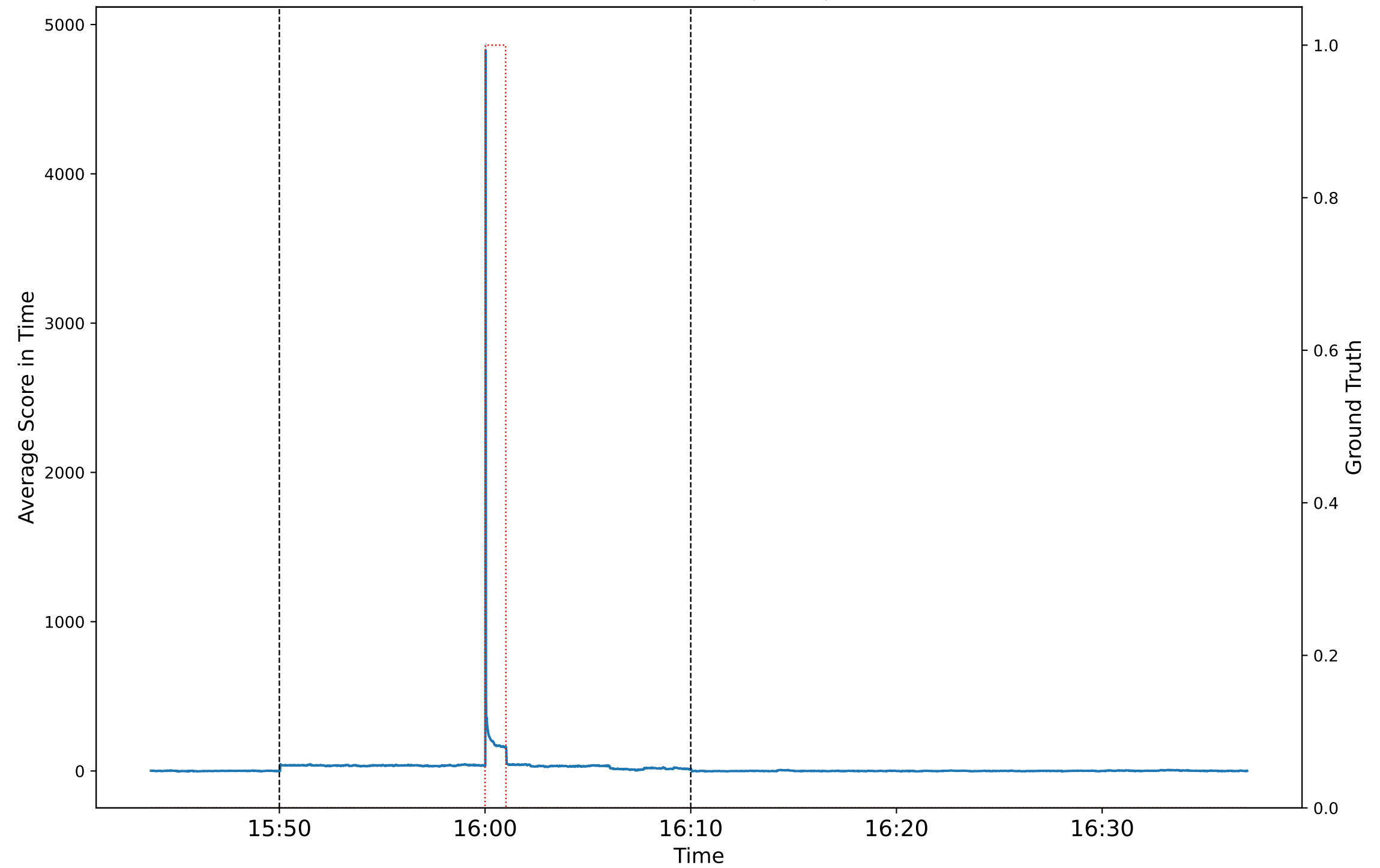
Score for OBKNN (TNone)
